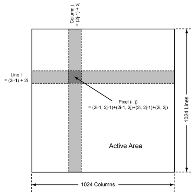
FIGURE 49. 2x2 Binning
